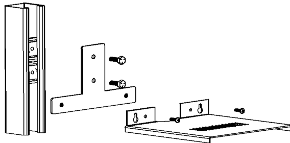
Exploded View of The Unistrut Method of Mounting the Shelf
