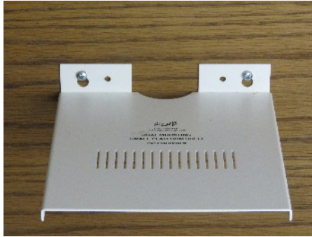
Shown Mounted to a Flat Surface
